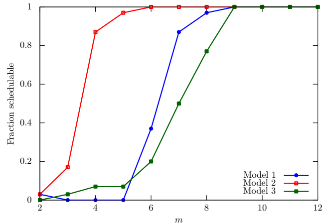
Fig. 2 Experimental results 2: percentage of task sets found to be schedulable by the three models. Variation of m ( \kappa = m , \bar{U} = 1 , p = 0.8 , \alpha = 0.2 ).
