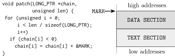
Figure 2: A possible implementation of the online patching mechanism performed by the detonator to make the ROP chain work in the presence of ASLR. LONG_PTR is a Windows signed data type used to represent native pointers.
