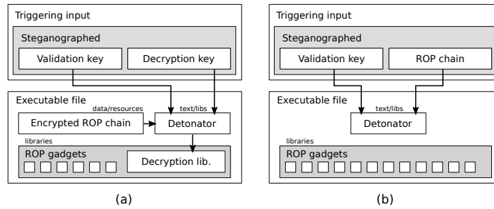
Figure 1: Implementation strategies: ROP chain embedded in (a) the executable file or (b) the input.
