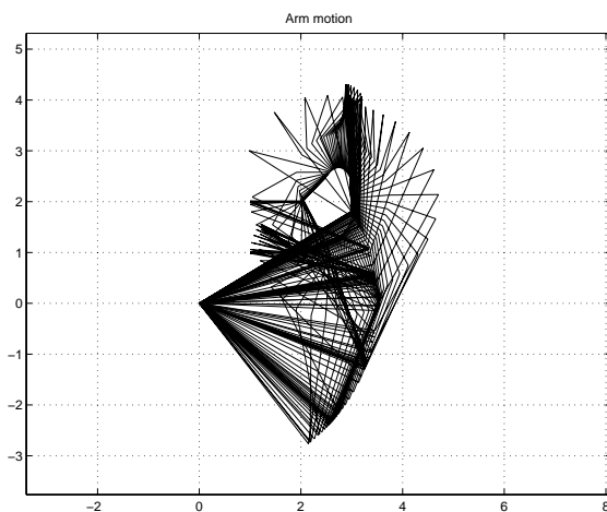
Fig. 6 Trajectory planning: stroboscopic motion of the (RR)_\alpha(RR)_u manipulator
